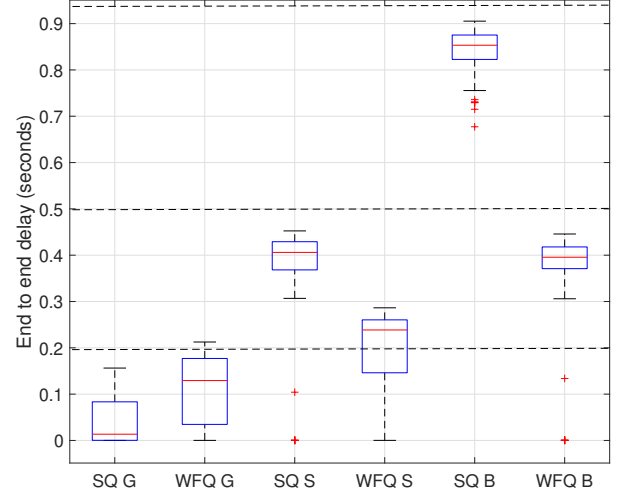
Figure 6: sLB and SQ vs sLB and WFQ: delay results. The removal of SQ leads to violations in gold flows’ delay results.
